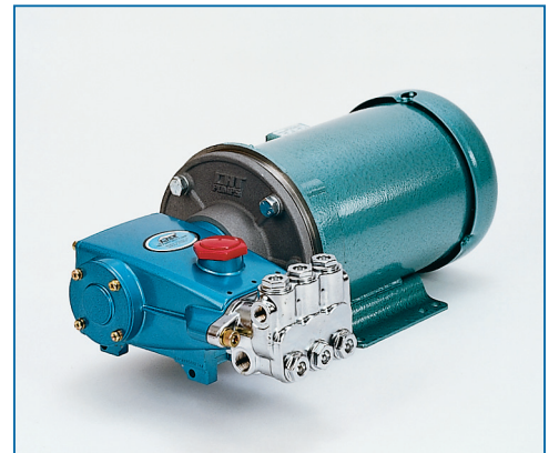
5FR BD Direct Drive
