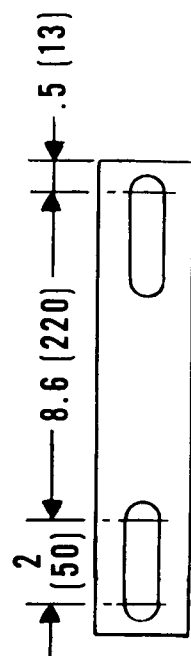
BOTTOM VIEW OF RAIL
